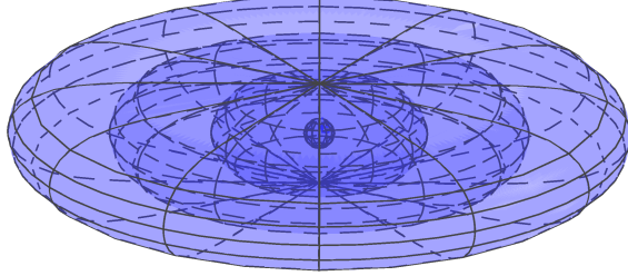
FIGURE 3. The rotationally symmetric ancient pancake. It shrinks to a round point as t \rightarrow 0 and sweeps out a slab of width \pi as t \rightarrow -\infty .
